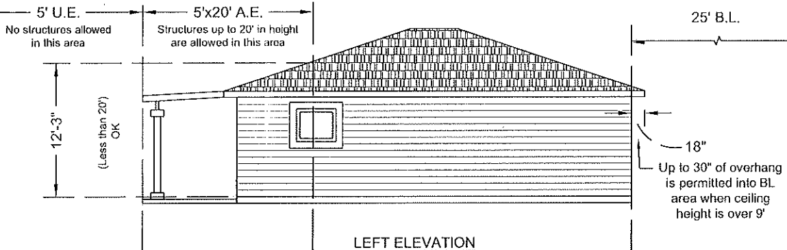
LEFT ELEVATION
