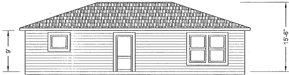
FRONT ELEVATION
